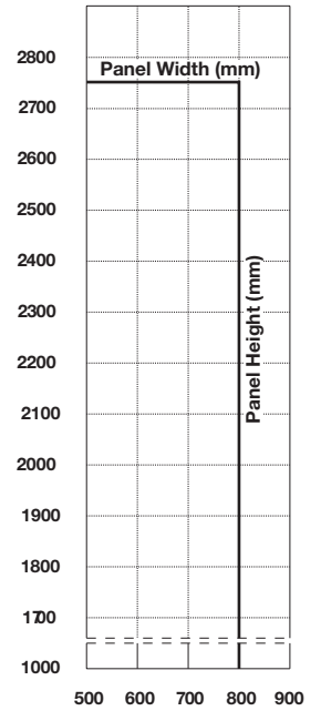
Panel Size Chart
